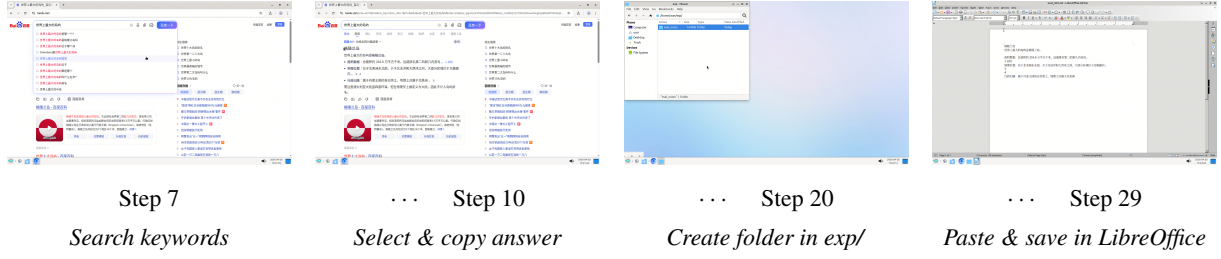
Figure 5: Browser Search demo (36 steps total). The agent searches for information in a browser, copies the answer, then switches to the file system to create a directory and file, and saves the content via LibreOffice—demonstrating cross-application coordination. The full trace is provided in Appendix E.2.
