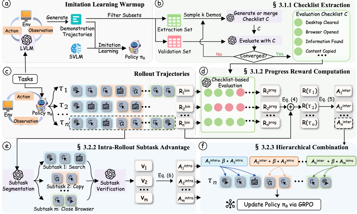
Figure 2: Overview of PAGE . Training begins with imitation learning warmup (a) and one-time checklist extraction (b). During RL, rollouts (c) are evaluated via checklist-based progress reward (d) and subtask-level completion verification (e), producing hierarchical advantages that are combined (f) for policy update.
