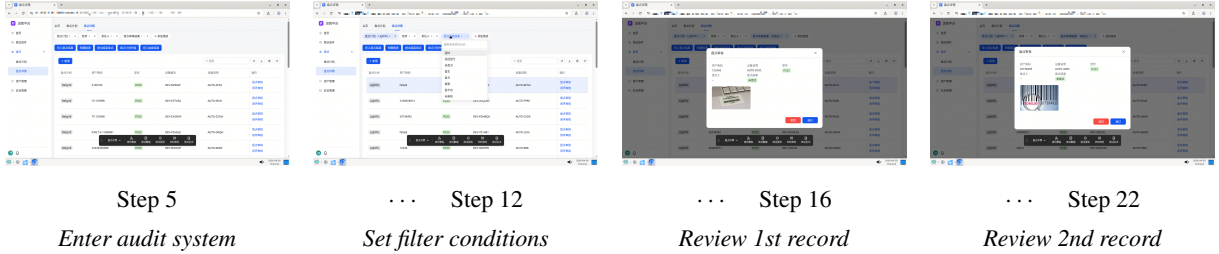
Figure 4: Asset Audit demo (25 steps total). The agent navigates a Web-based asset management system, sets filter conditions, then reviews each record by comparing the photo barcode against the system barcode to make pass/reject decisions. The full trace is provided in Appendix E.1.
