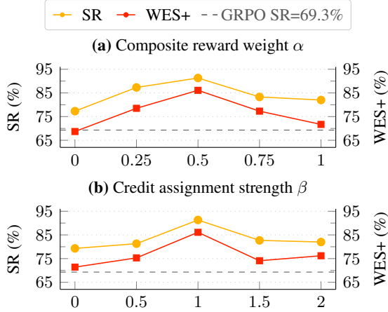
Figure 3: Hyperparameter sensitivity on Asset Audit. (a) \alpha controls composite reward weight (Eq. (4)). (b) \beta controls intra-rollout subtask advantage strength (Eq. (7)). Both metrics peak at \alpha=0.5 , \beta=1.0 .
