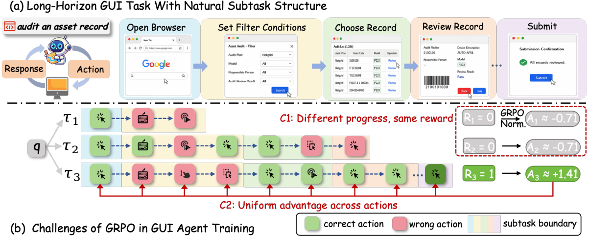
Figure 1: (a) A long-horizon GUI task naturally composed of semantically complete subtasks. (b) Two limitations of GRPO on long-horizon GUI tasks: rollouts with different progress receive the same reward (C1), and all actions within a rollout receive uniform advantage regardless of correctness (C2).
